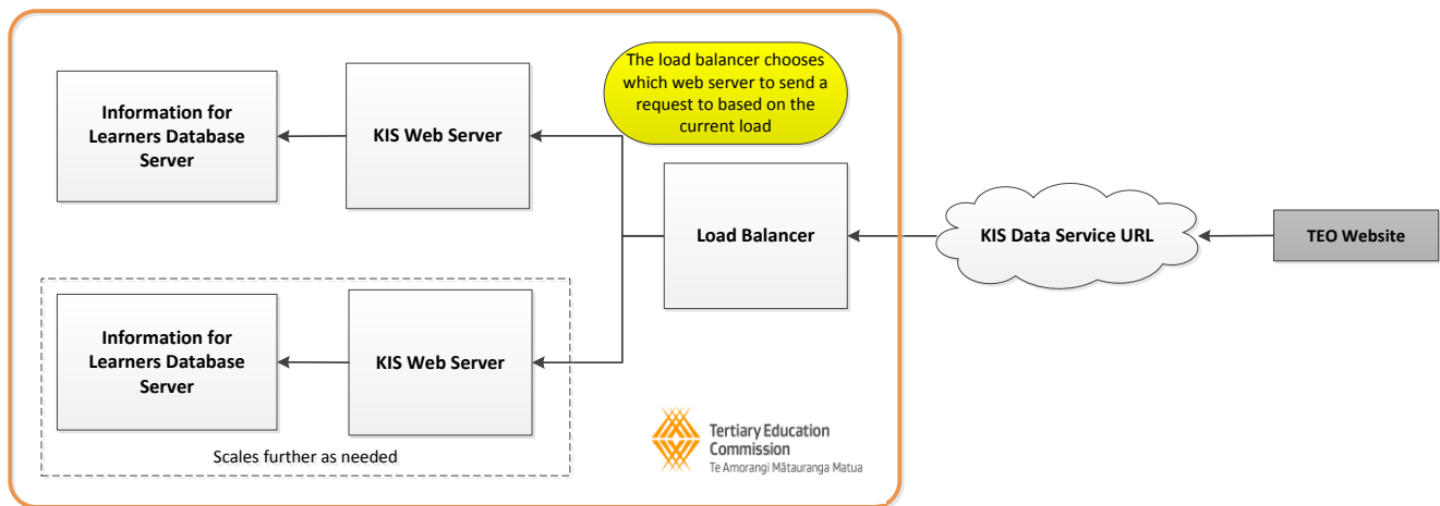
Figure 2: Server configuration showing load balancing for the KIS Production environment
